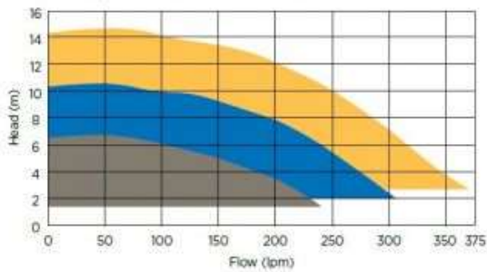
Supatuf ECO MK2 100 Performance Curves
