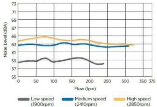
Supatuf ECO MK2 100 Noise Levels
