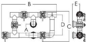
5 Way Butterfly Valve NBV30-NBV80
